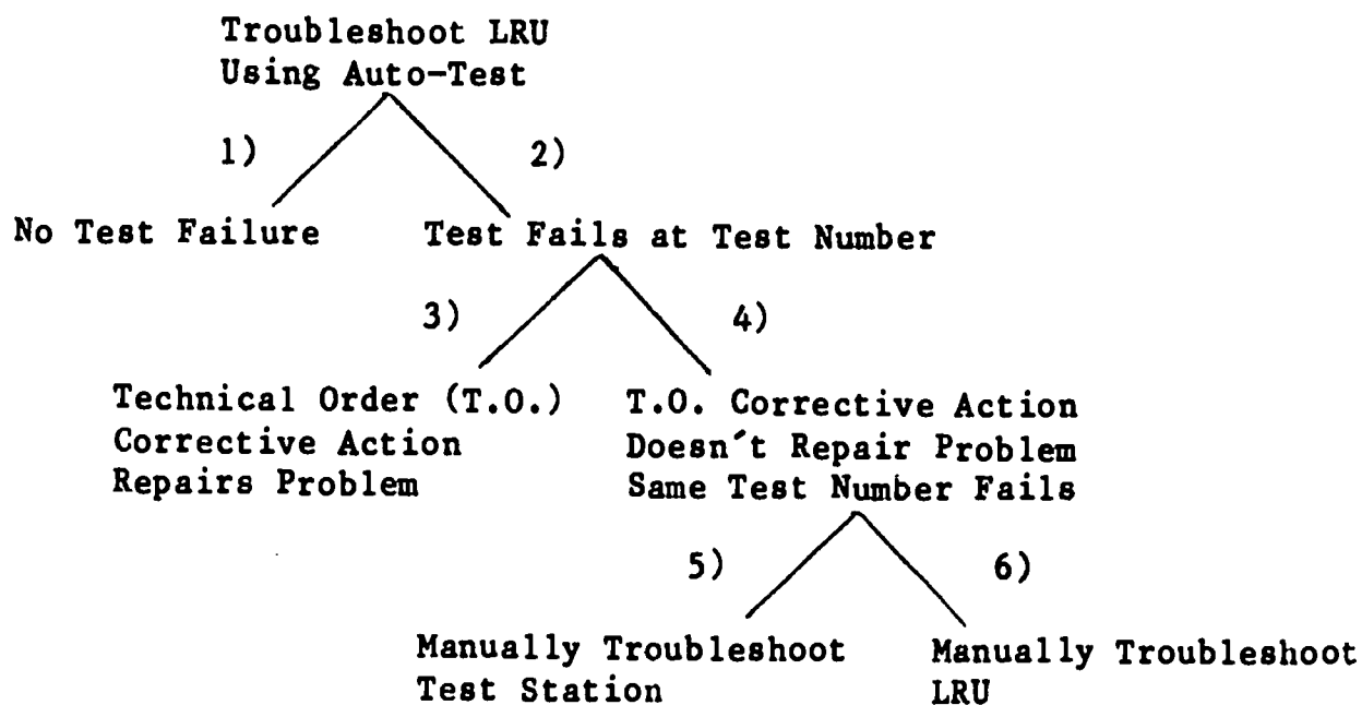
Figure 6. Job Logic.
